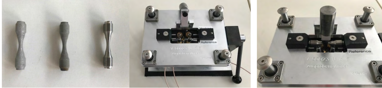
Figure 1 —Photo of AM samples and PCRT fixture
